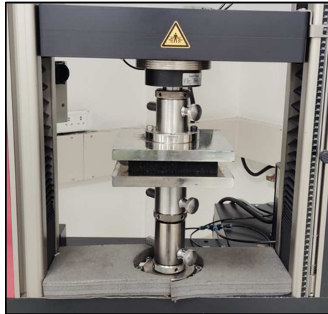
Setup photograph
